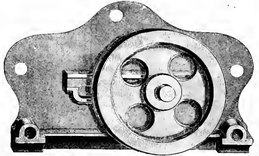
Fig. 2834a. Side Elevation, with one Side-plate removed. "ANTI-FRICTION" CAR-DOOR SHEAVE.
